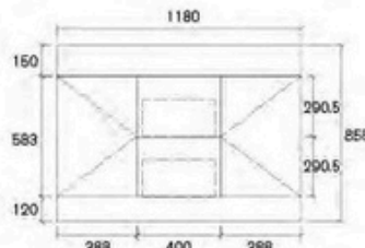
AELIZA-1200WD-SD Size: 1180x450x855mm
