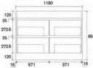
AJ04-1200SA2-SD(SINGLE BOWL) Size: 1180x450x855mm
