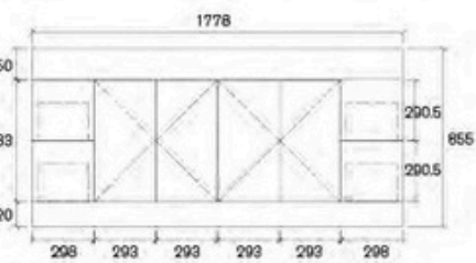
AELIZA-1800W-SD Size: 1778x450x855mm
