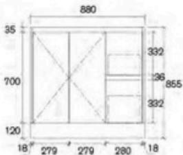
ASIE-900W-SD Size: 880x355x855mm
