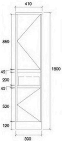
ASK6BA2 Size: 410x400x1800mm
