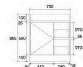
ATB-750RA1-SD Size: 730x450x855mm
