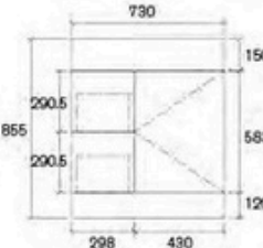
AELIZA-750WL-SD Size: 730x450x855mm
