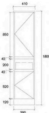
ASK7B Size: 410x400x1800mm
