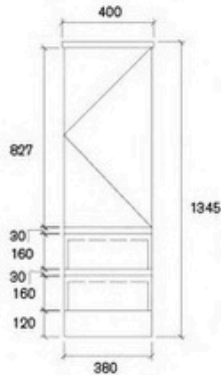
ASK16ADWA2 Size: 400x400x1345mm
