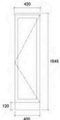
ASK16A Size: 420x400x1545mm
