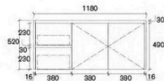
ARYE-1200LA2-SD Size: 1180x455x520mm
