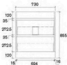
AJ04-750A2-SD Size: 730x450x855mm
