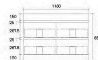
ACV-1200WD-CM (DOUBLE BOWL)
