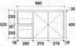
AL76-900WL-S-D Size: 880x455x520mm
