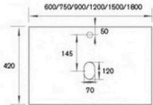
Single bowl standard cutout 420mm depth
