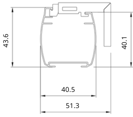
Bead Chain/ Motorized Headrail Screw Fix
